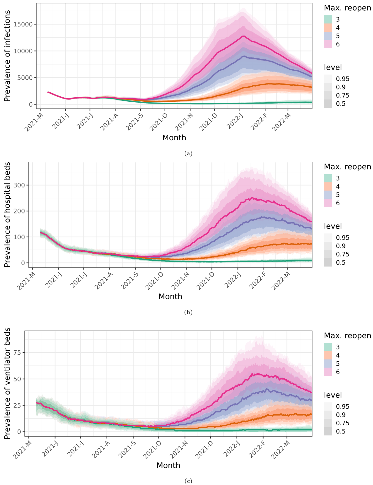
Figure 7: Long-term predictions for prevalence (a), hospital beds (b) and ventilator beds (c). Each color shows the scenario of one reopening factor, 3, 4, 5 and 6.
