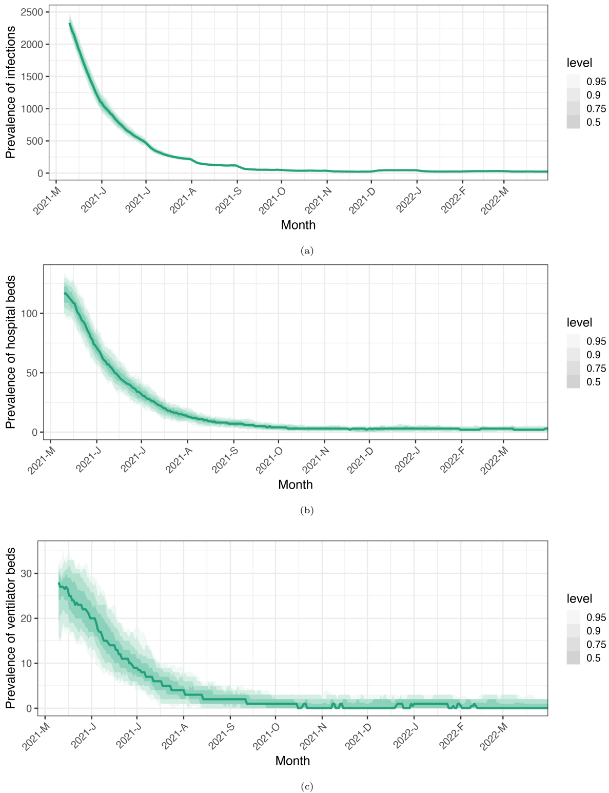
Figure 6: Long-term predictions for prevalence (a), hospital beds (b) and ventilator beds (c). The monthly variation in the prevalence of infections is mainly contributed by the numbers of imported cases.
