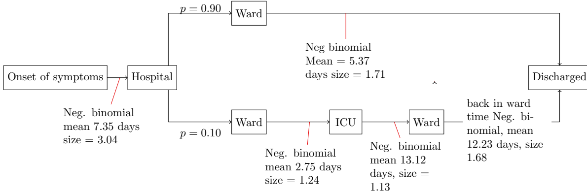
Figure 29: Hospital assumptions and parameters used between 1 June 2020 and 1 January 2021
