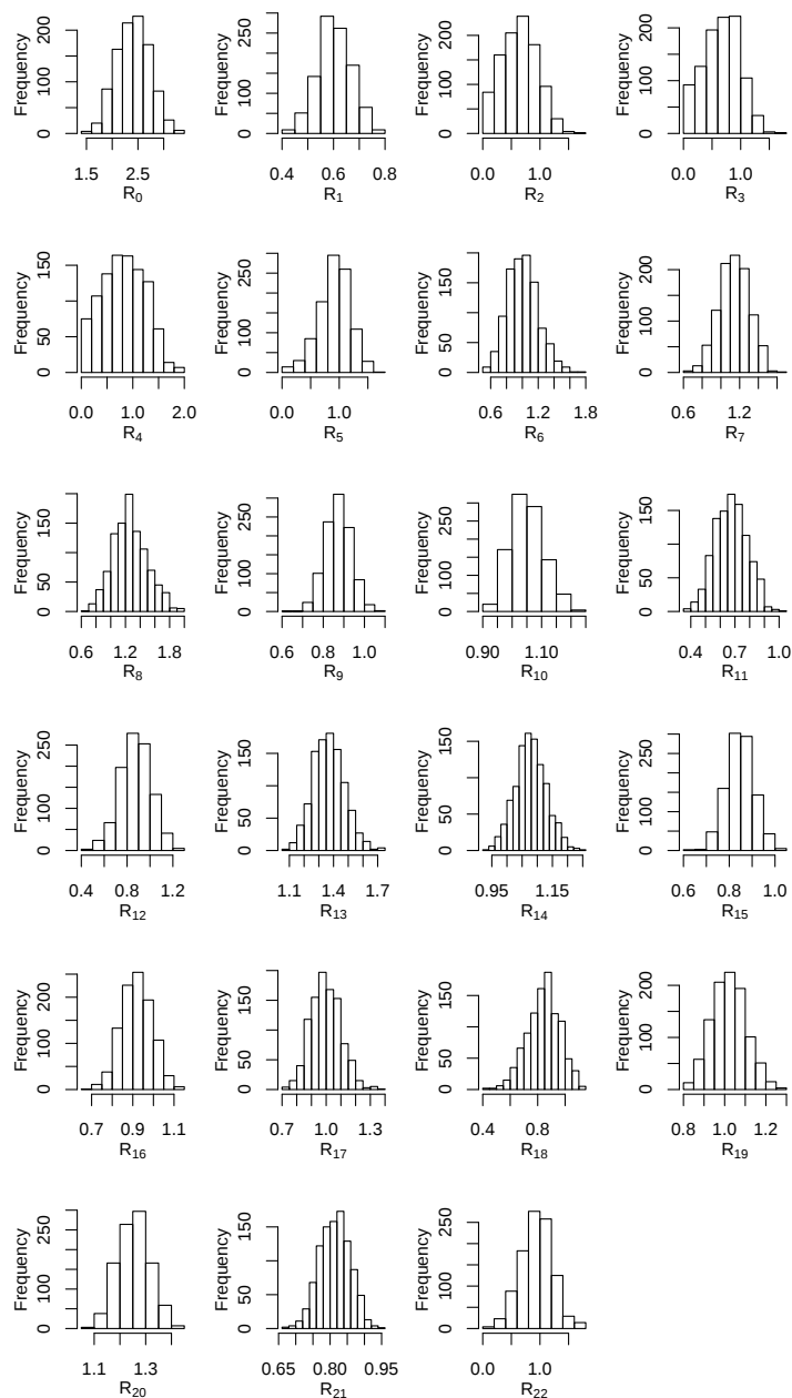
Figure 33: Estimated densities of the reproduction numbers. National model
