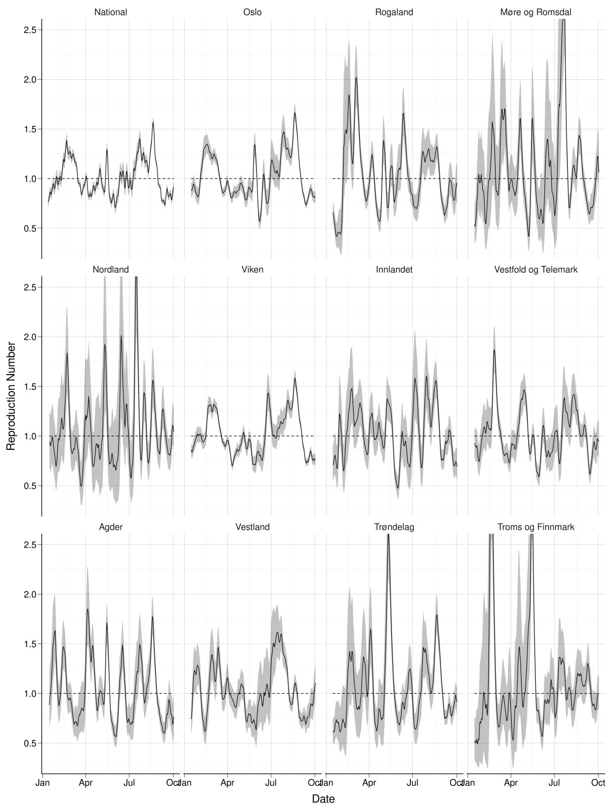
Figure 34: Reproduction number estimated using the R package EpiEstim.
