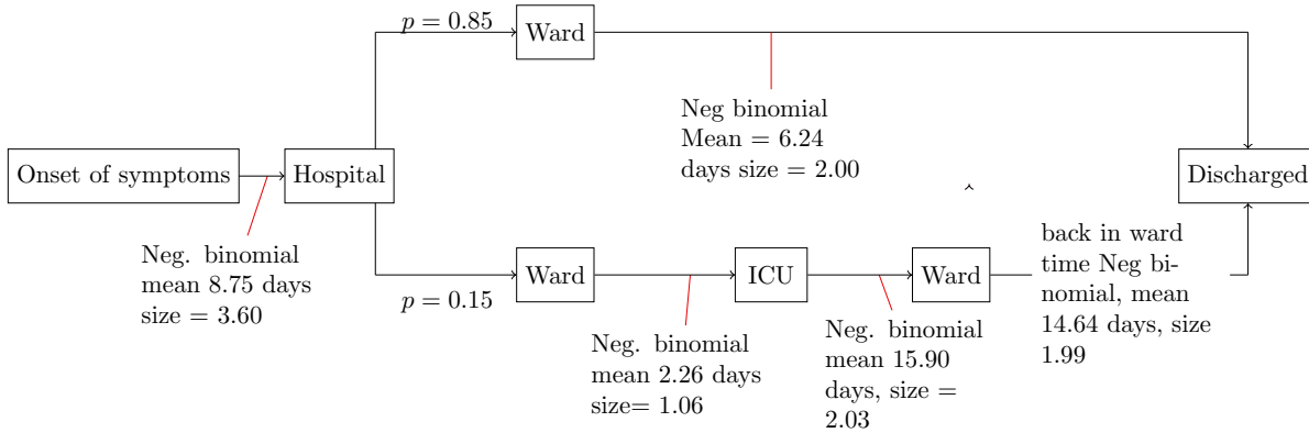
Figure 28: Hospital assumptions and parameters used before 1 June 2020
