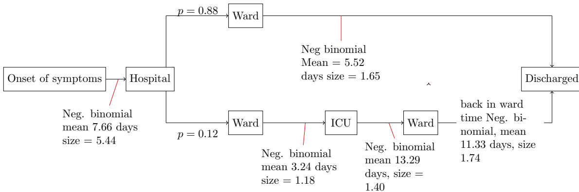
Figure 30: Hospital assumptions and parameters used between 1 January 2021 and 1 March 2021
