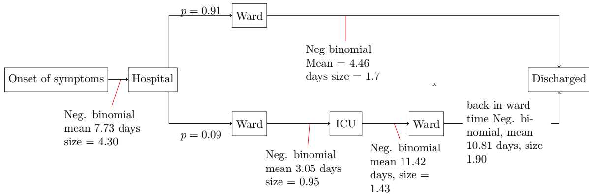
Figure 32: Hospital assumptions and parameters used from 1 June 2021
