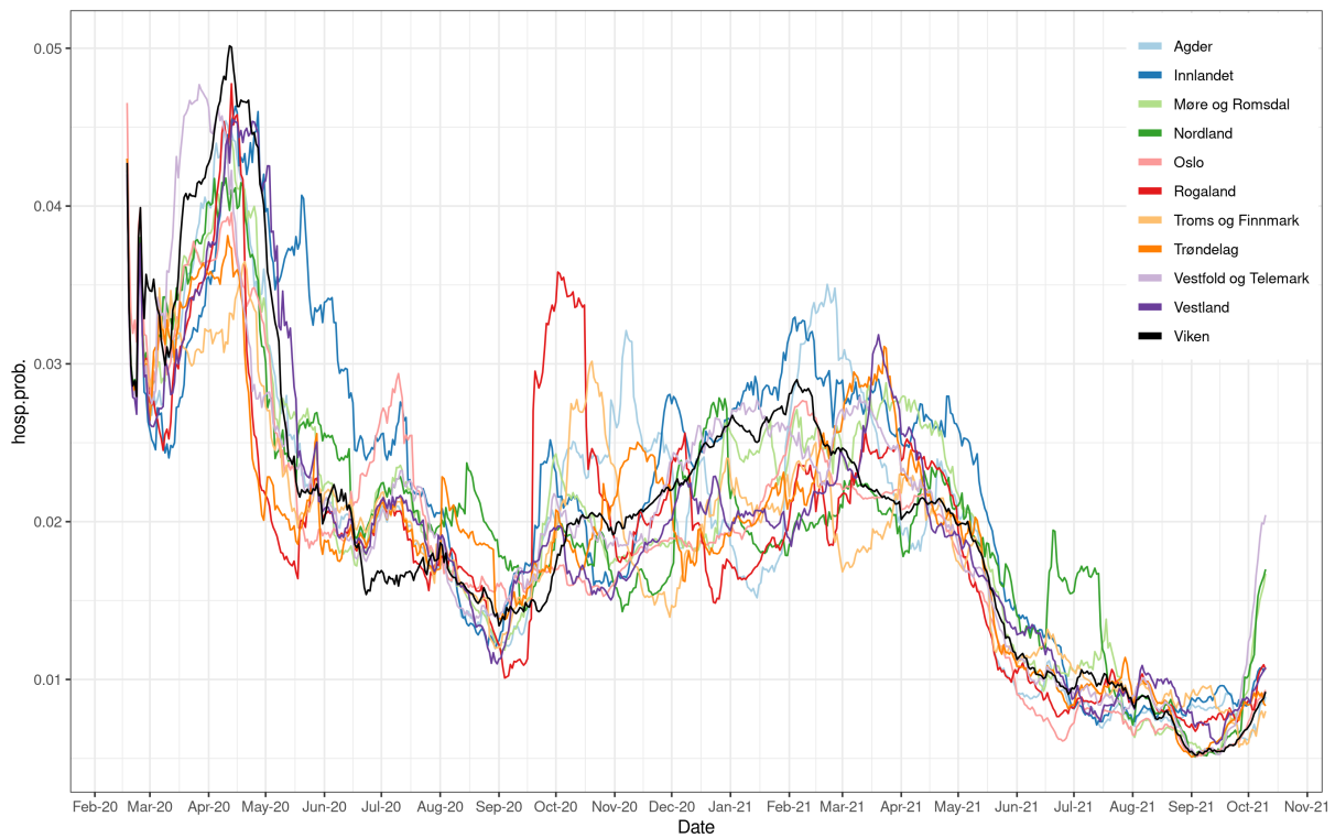
Figure 35: Regional hospitalization probabilities per infection. The estimates are based on Salje et al., and regional data on the age distribution in the test data and the empirical case-hospitalisation rates.
