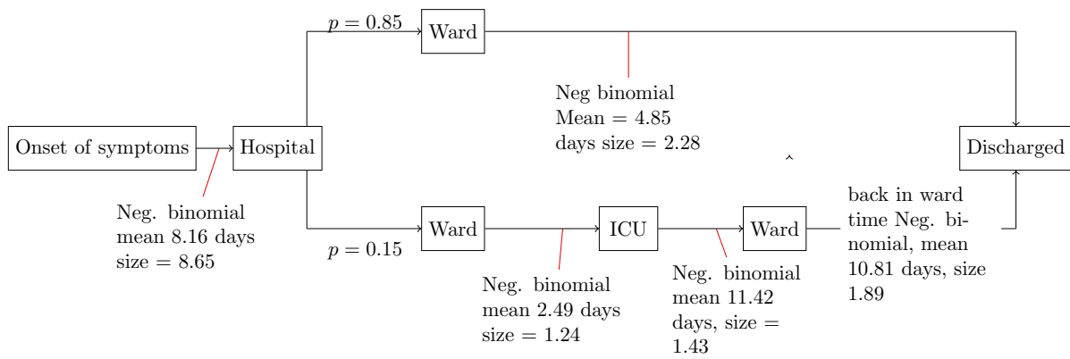
Figure 31: Hospital assumptions and parameters used between 1 March 2021 and 1 June 2021
