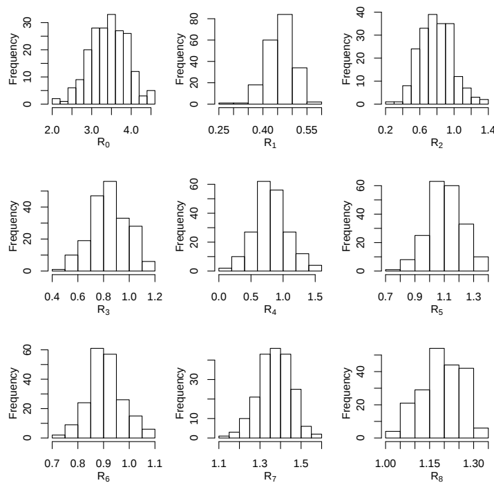
Figure 30: Estimated densities of the reproduction numbers. National model
