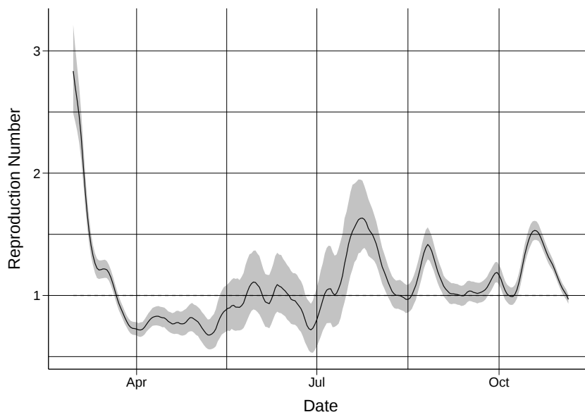
Figure 31: Reproduction number estimated using the R package EpiEstim.
