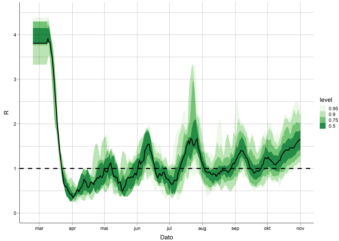
Figure 3: R(t) estimates until 14 days ago using a Sequential Monte Carlo (SMC) approach calibrated to incidence data. The large uncertainty during the last 14 days reflects the lack of available data due to the time lag between infection, symptoms onset and hospitalisation. Therefore we omit the plot of the last 14 days. The green band shows the 95% posterior confidence interval. We observe that R(t) dropped below 1 in the middle of March, corresponding to the lockdown. It remained stable around 0.5 until the end of April, when it increased to 1 in the beginning of May. It then kept oscillating below and above 1, in accordance with increases and decreases of the number of new hospitalisations. R(t) is sensitive to these oscillations in the data. An increase in hospital admissions indicates a daily reproduction number (14 days before on average) above 1. A decrease in hospital admissions suggests that the reproduction number was below 1 (again 14 days prior).
