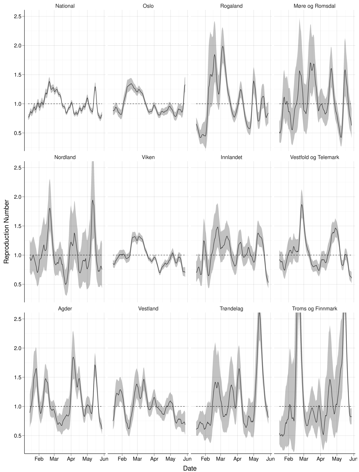
Figure 37: Reproduction number estimated using the R package EpiEstim.
