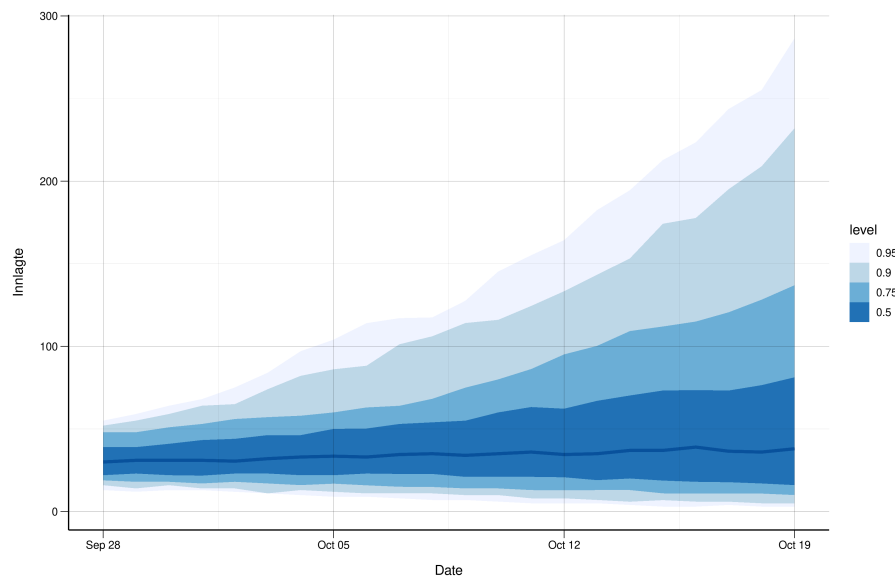
Figure 8: Predicted daily number of COVID-19 patients in hospital in Norway (95% confidence intervals and interquartile range), next three weeks, including patients ventilator treatment.
