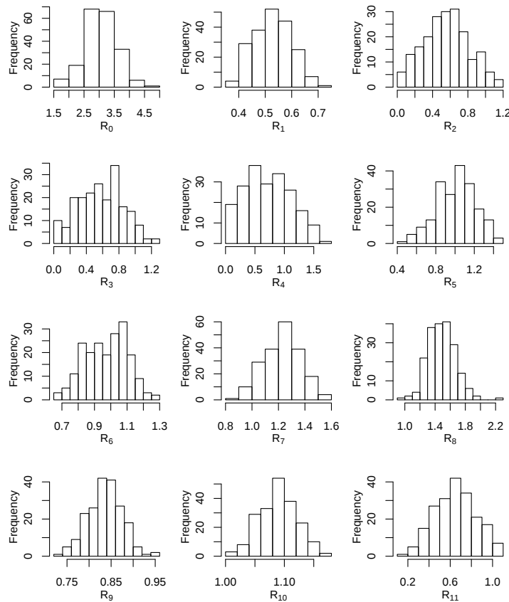
Figure 32: Estimated densities of the reproduction numbers. National model
