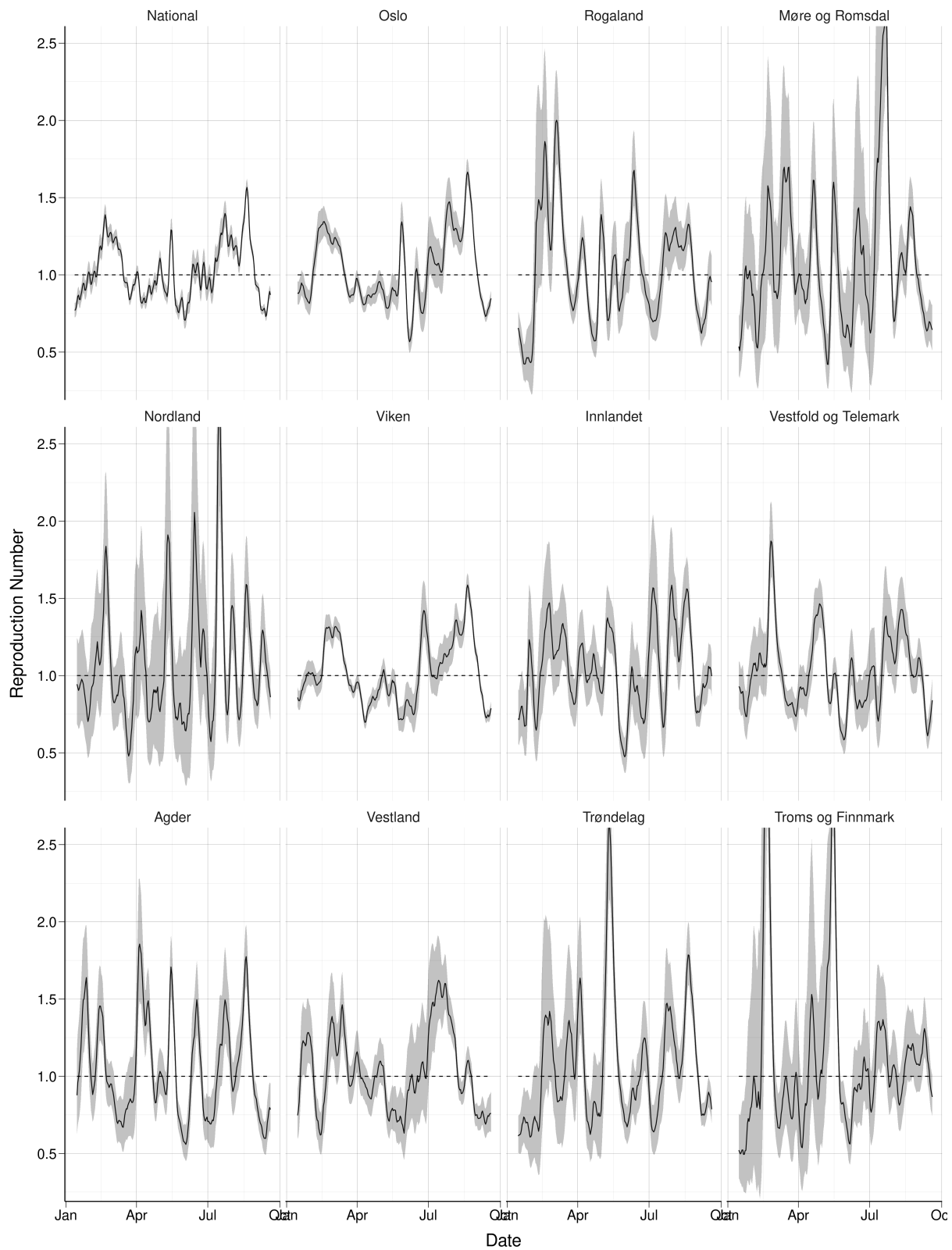
Figure 17: Reproduction number estimated using the R package EpiEstim.
