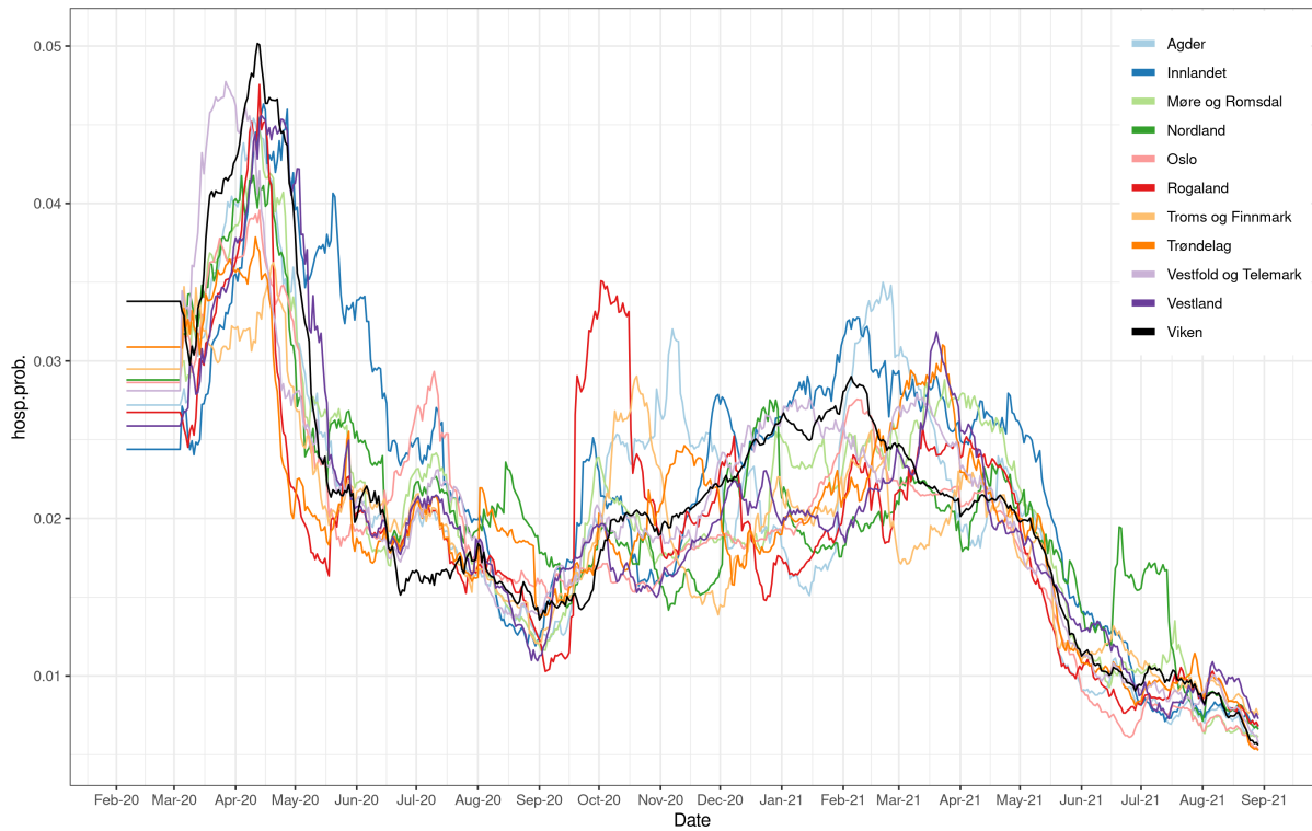
Figure 18: Regional hospitalization probabilities per infection. The estimates are based on Salje et al., and regional data on the age distribution in the test data and the empirical case-hospitalisation rates.
