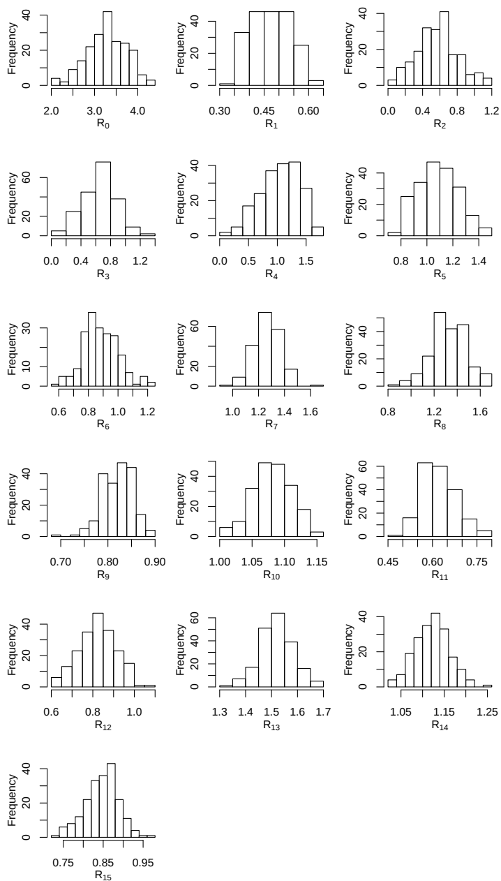
Figure 35: Estimated densities of the reproduction numbers. National model
