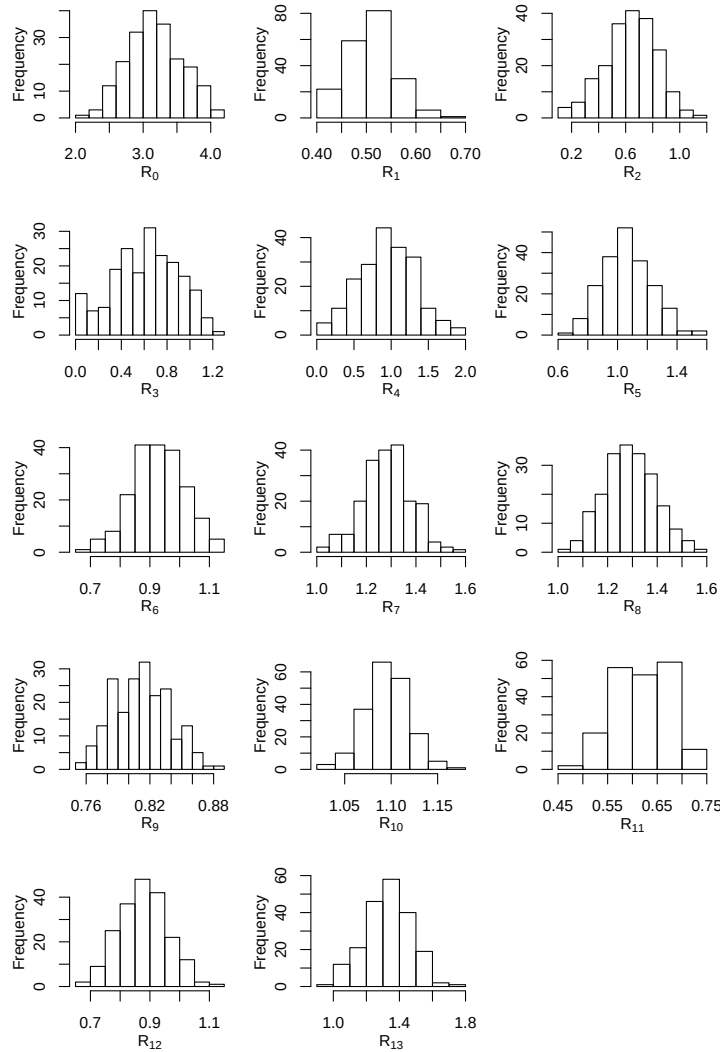
Figure 36: Estimated densities of the reproduction numbers. National model
