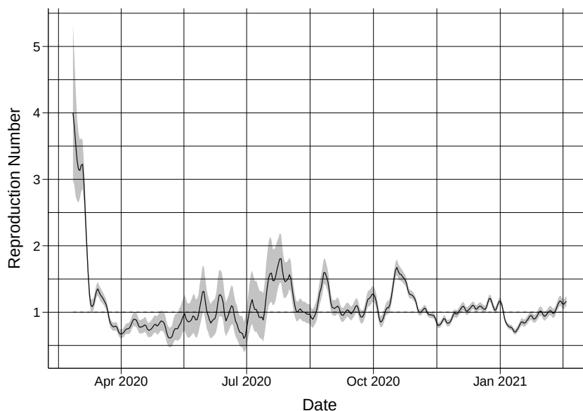
Figure 37: Reproduction number estimated using the R package EpiEstim.
