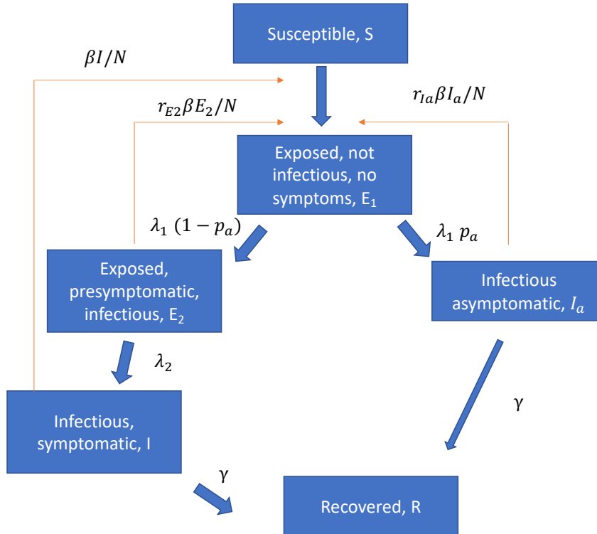
Figure 15: Schematic overview of the model.
