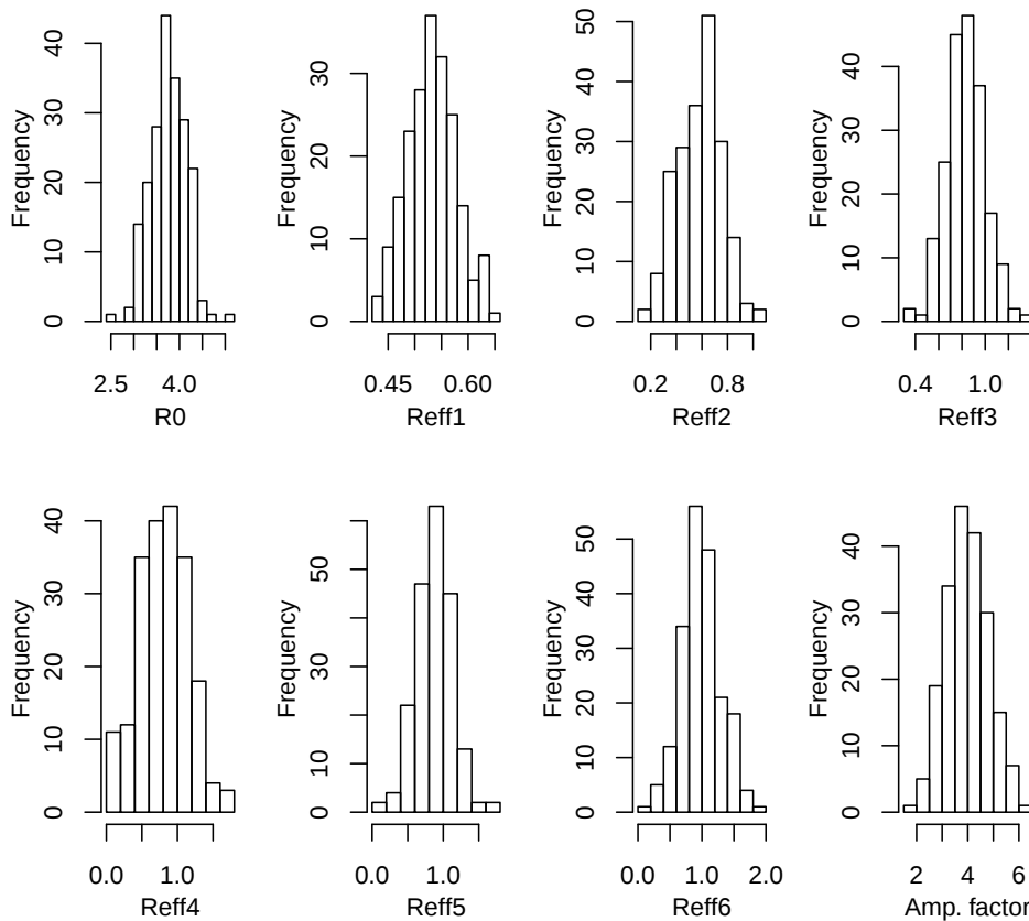
Figure 1: Estimated densities of the eight parameters.
