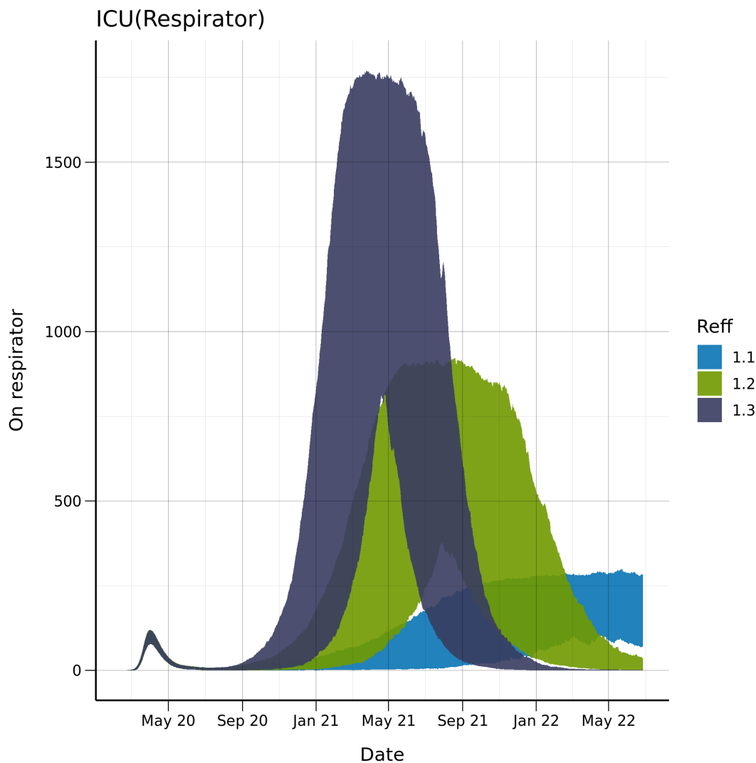
Figure 18: Predicted number of COVID-19 patients needing ventilator treatment based on three different scenarios with R_{\text{effective}} equal to 1.1, 1.2 and 1.3.
