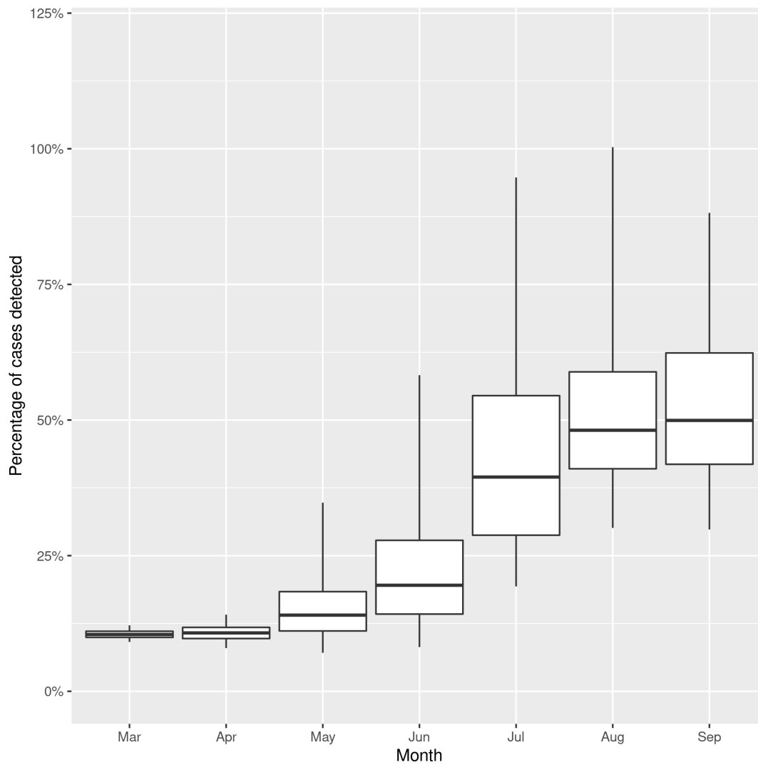
Figure 6: Percentage of cases detected through testing according to the model over time. The randomness shown in the 95% confidence intervals accounts only for the uncertainty in the parametrisation of the model. The confidence intervals do not account for the uncertainty about the infection rate. Test results are also prone to mistakes, which are not modelled here. The results should be interpreted with caution.
