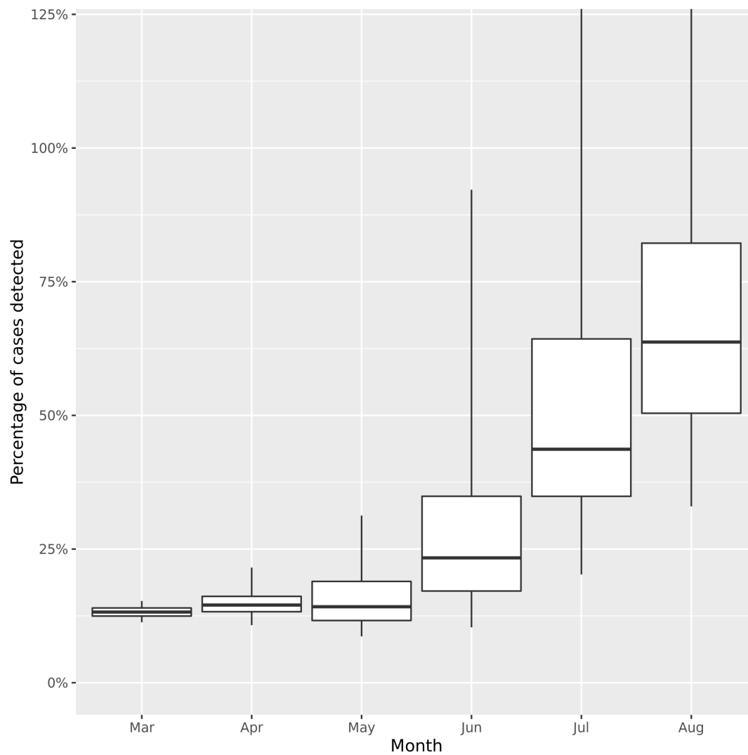
Figure 6: Percentage of cases detected through testing according to the model over time. The randomness shown in the 95 % confidence intervals accounts only for the uncertainty in the parametrization of the model. The confidence intervals do not account for the uncertainty about the infection rate. Test results are also prone to mistakes, which are not modelled here. The results should be interpreted with caution,
