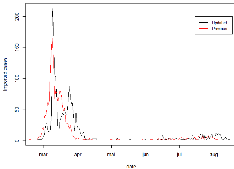
Figure 20: Comparison between the number of imported cases on the day of declared appearance of symptoms (red) and on the date of positive test, which is used from now on (black).
