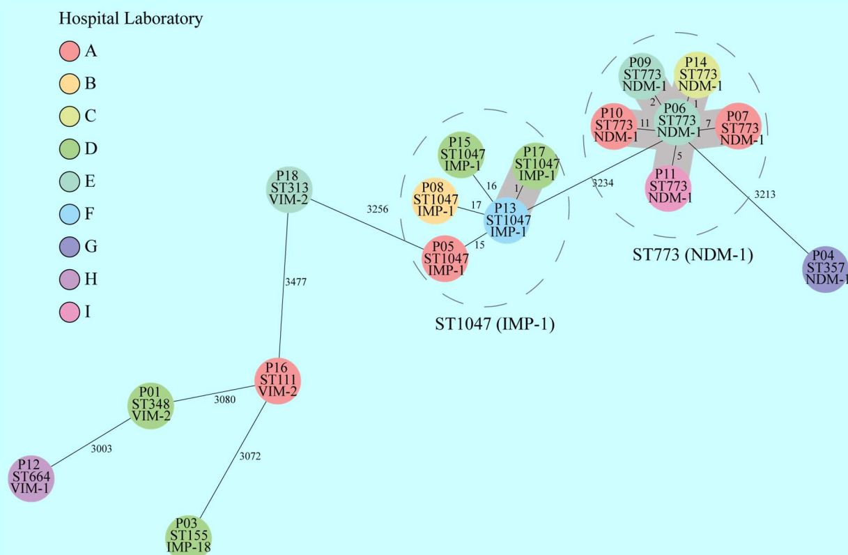
FIGURE 97. Minimum spanning tree of carbapenemase-producing P. aeruginosa isolates in 2022 based on 3,867 core genome alleles using SeqSphere+. Each circle represents one isolate (P01 to P18) and the colour codes the laboratory where the isolate was identified (A to I). The STs and carbapenemase variants are indicated. The number of allelic differences is shown along the lines. Closely related isolates ( \leq 12 allelic differences) are highlighted with grey shading.
