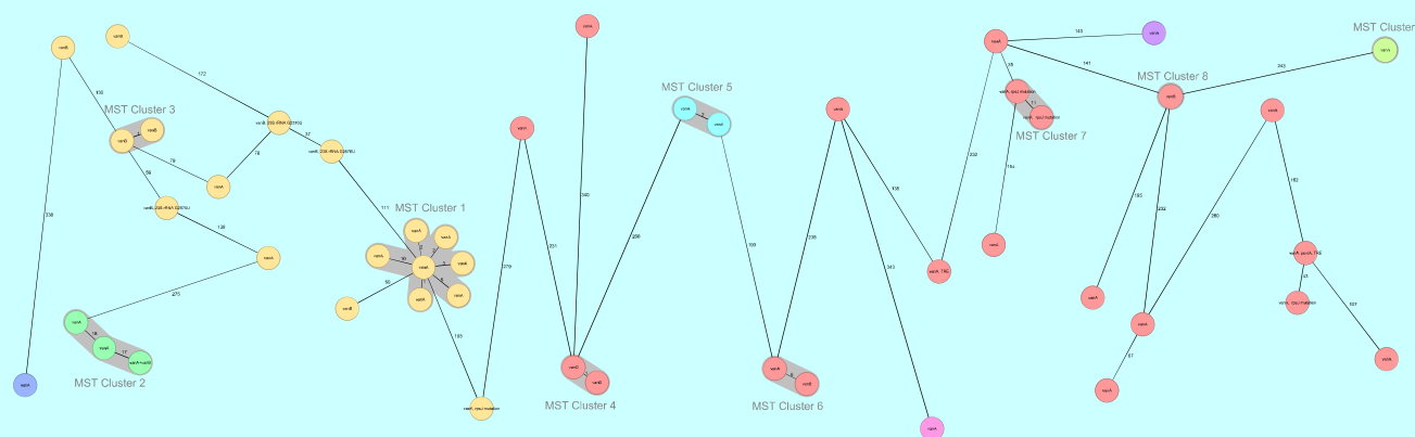
FIGURE 108. Minimum spanning network built from core genome allelic profiles of 49 Norwegian VRE E. faecium 2022 isolates using Ridom-SeqSphere+ software with integrated core genome (cg) MLST scheme with E. faecium Aus0004 as reference strain. The isolates are colour-coded according to sequence type. VRE, LRE and tigecycline resistance is indicated in the circles. Isolates with zero allelic differences end up in the same circle. The number of allelic differences between isolates is indicated on lines between the circles. Nine different clusters ( \leq 20 allelic differences) are highlighted with grey markings.
