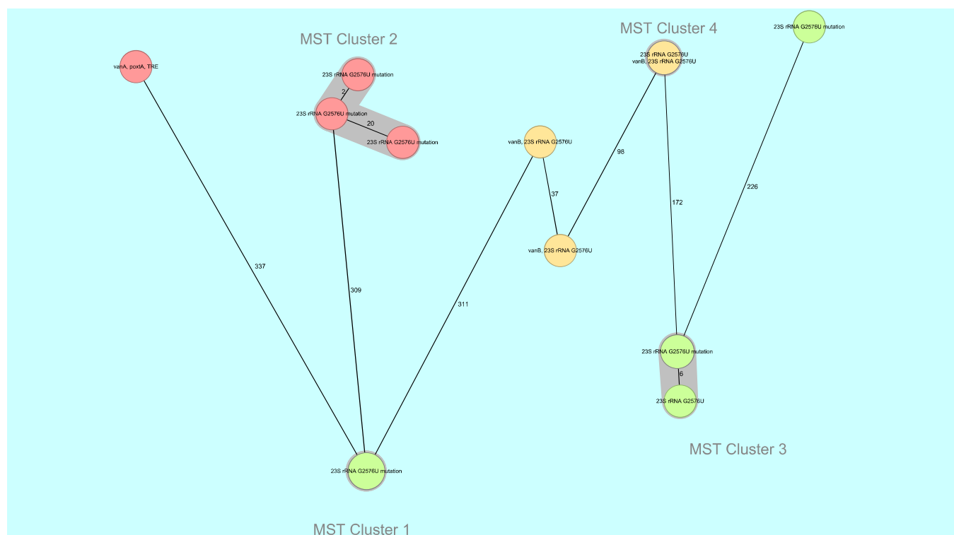
FIGURE 113. Minimum spanning network built from core genome allelic profiles of the 16 Norwegian LRE E. faecium 2022 isolates using Ridom-SeqSphere+ software with integrated cgMLST scheme with E. faecium Aus0004 as reference strain. The isolates are colour-coded according to ST. Two isolates showed identical allelic profiles and are thus not showed as separate circles. VRE, LRE and tigecycline resistance is indicated in the circle. Number of allelic distances between the isolates are given at the lines between the circles. Four clusters with \leq 20 allelic distances are highlighted with grey marking.
